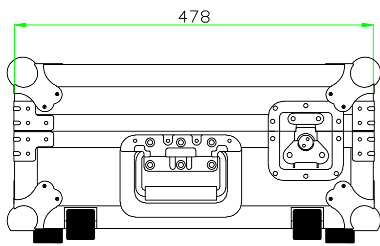
LEFT VIEW
