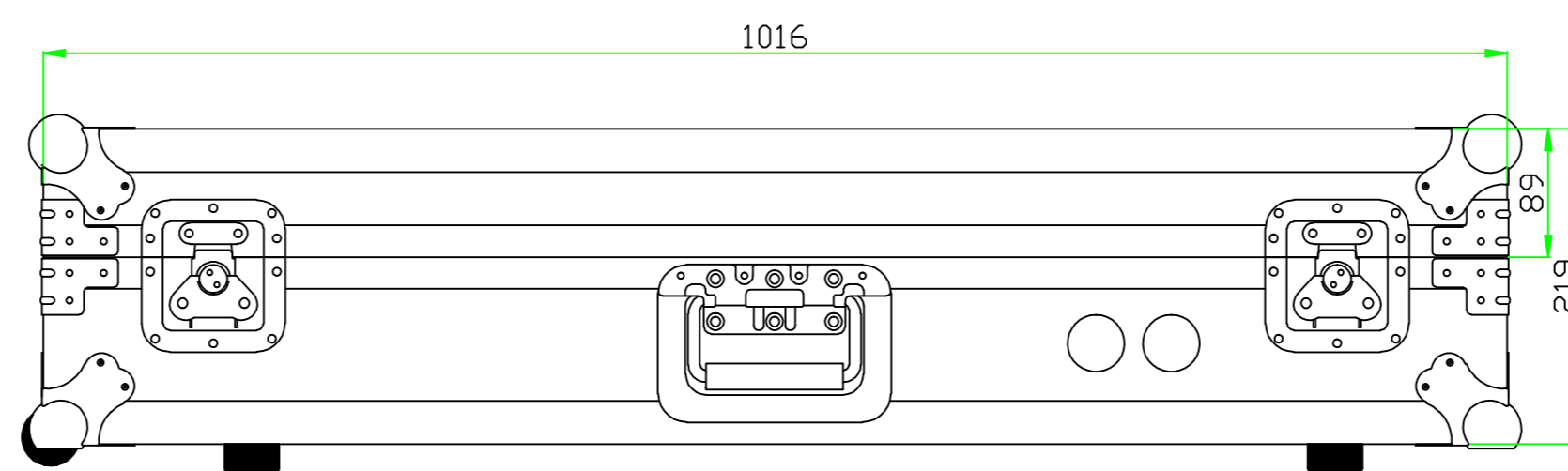
BACK VIEW
