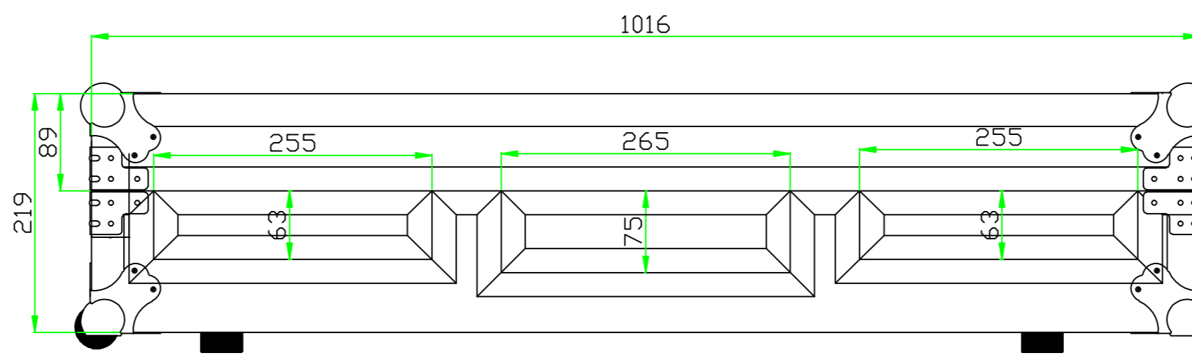
FRONT VIEW
