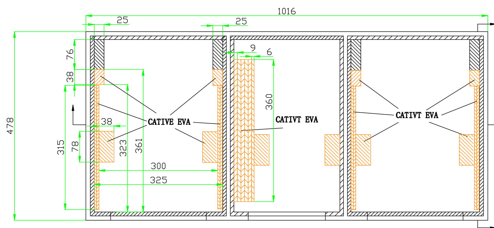
TOP VIEW OF BASE
