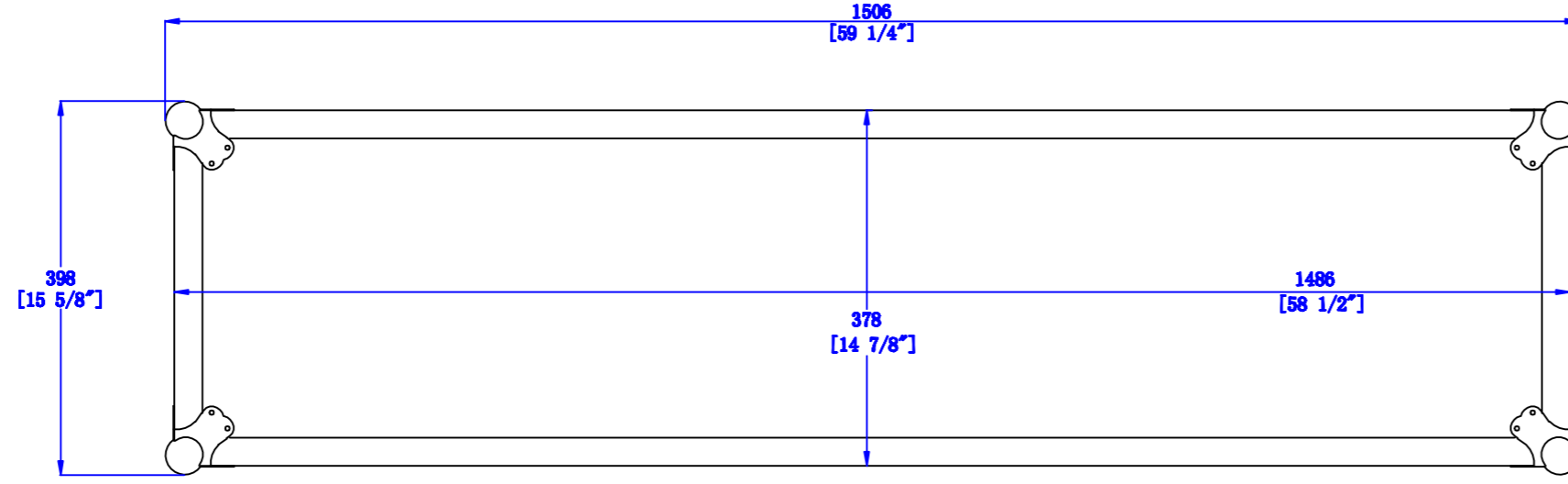
TOP VIEW
