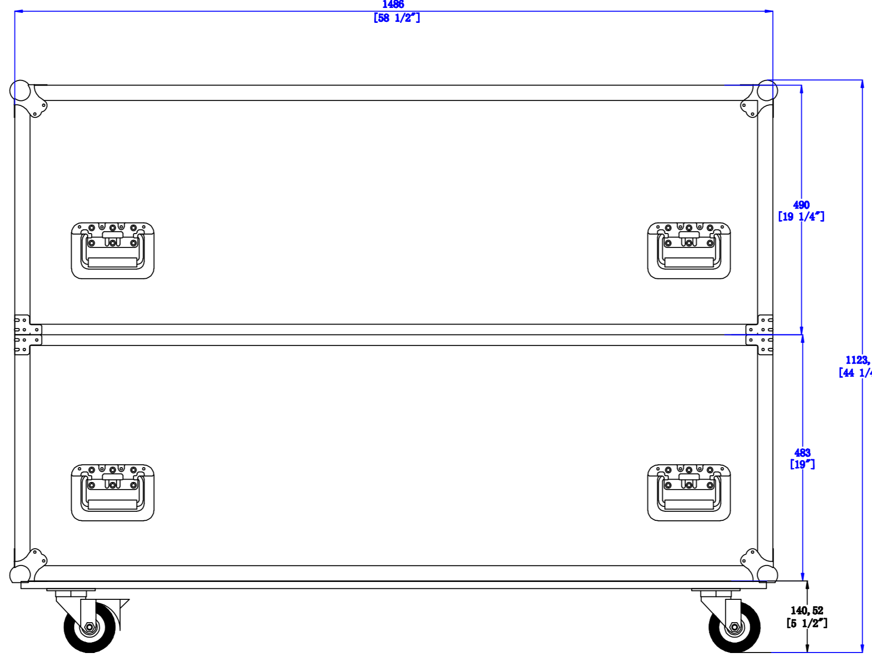
FRONT VIEW
