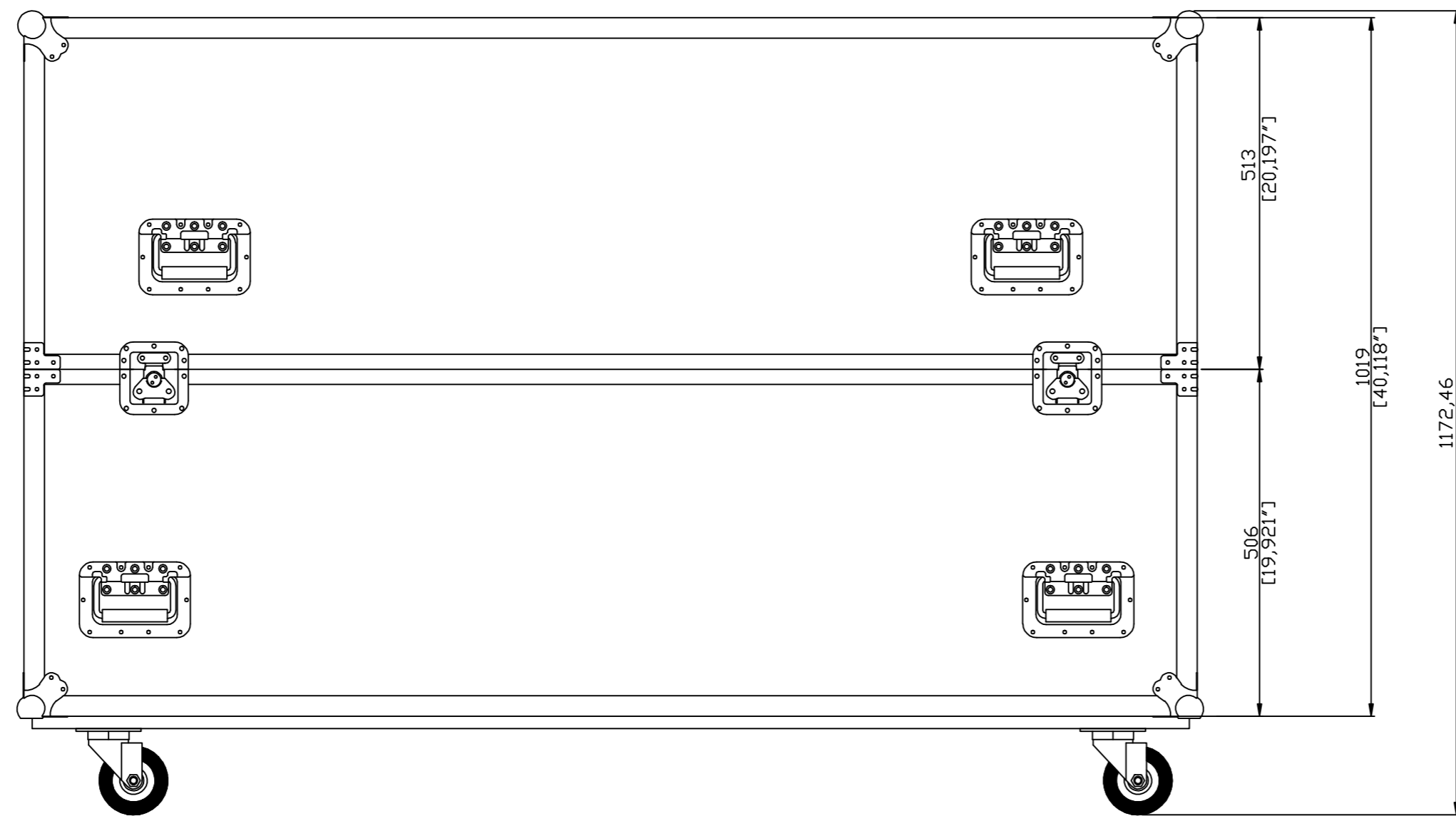
FRONT&BACK VIEW
