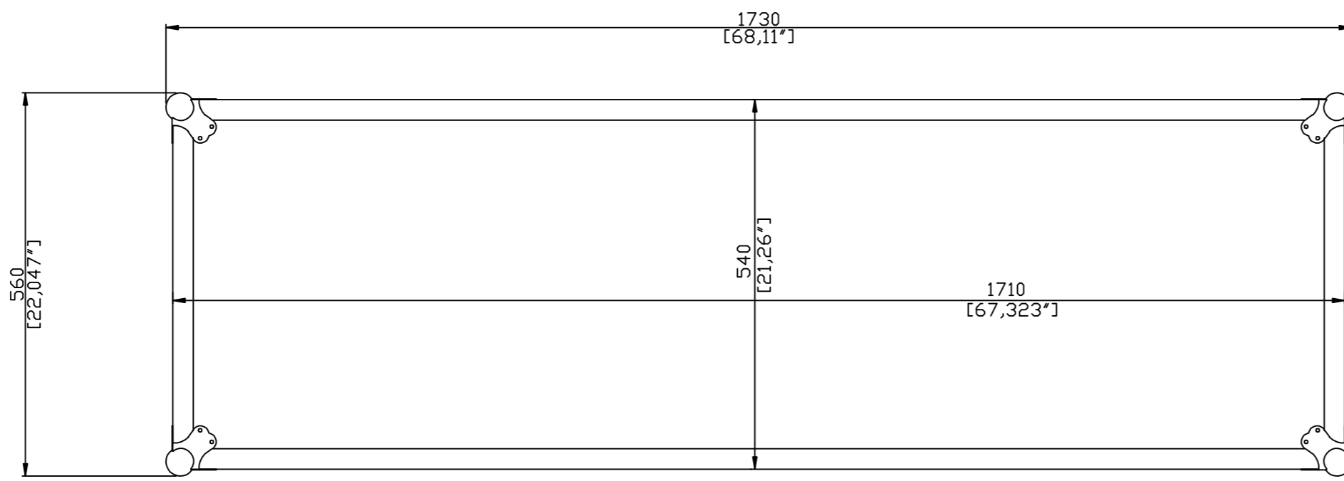
TOP VIEW
