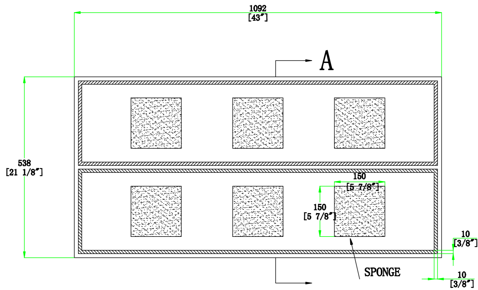
BOTTOM VIEW OF COVER
