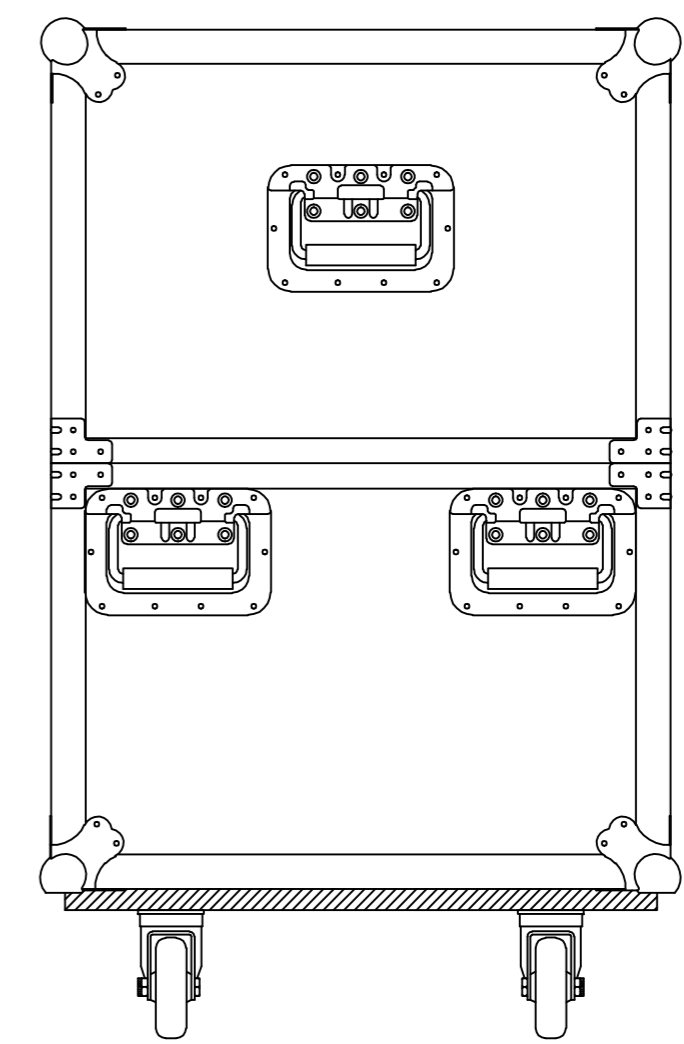
LEFT&RIGHT VIEW
