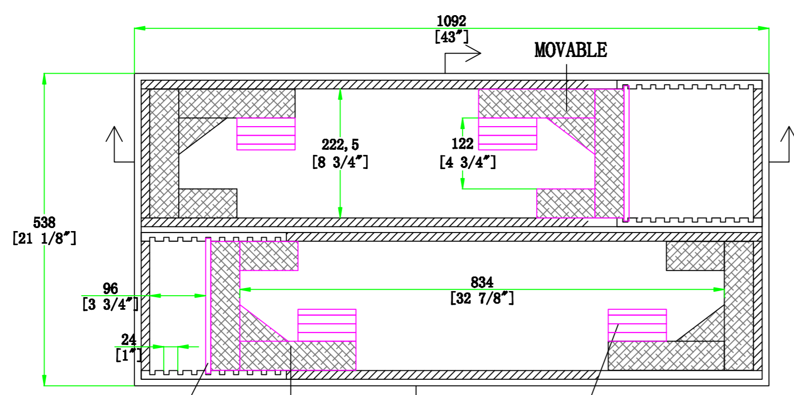
TOP VIEW OF BASE
